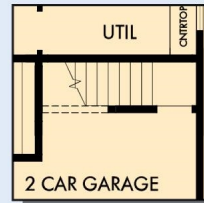
FIRST FLOOR WITH OPTIONAL SECOND FLOOR WALK-UP STORAGE
