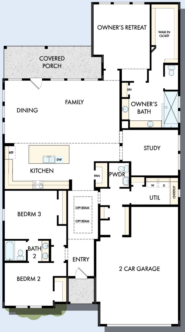
FIRST FLOOR WITH OPTIONAL SECOND FLOOR WALK-UP STORAGE
