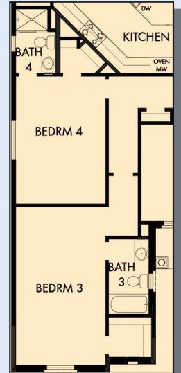
OPTIONAL EXTENDED BEDROOM 3 AND 4 WITH BATH 4
