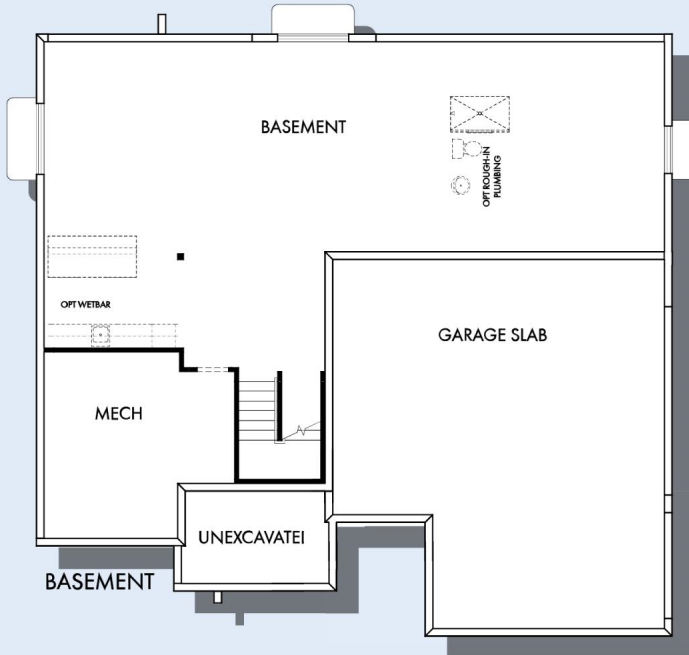
OPTIONAL SIDE DAYLIGHT BASEMENT
