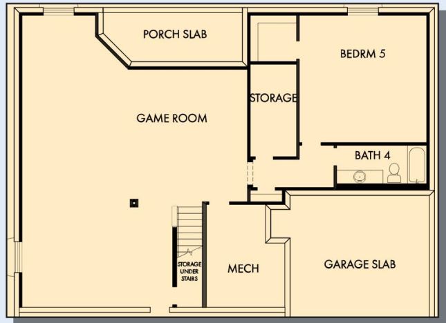
OPTIONAL GAME ROOM WITH BEDROOM 5 AND BATH 4 AT BASEMENT
