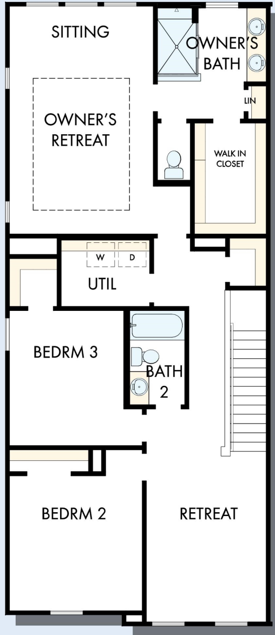
SECOND FLOOR
