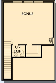
OPTIONAL SECOND FLOOR BONUS WITH HALF BATH
