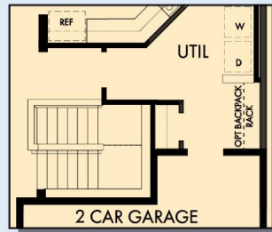
FIRST FLOOR WITH OPTIONAL BASEMENT
