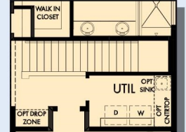
FIRST FLOOR WITH OPTIONAL FINISHED BASEMENT
