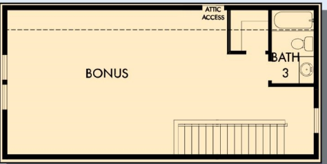
OPTIONAL SECOND FLOOR BONUS WITH BATH 3
