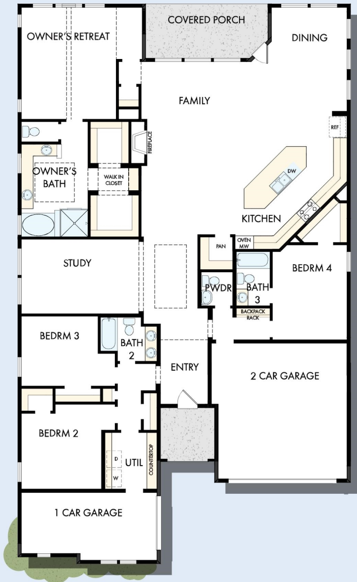
OPTIONAL EXTENDED COVERED PORCH AT FAMILY
