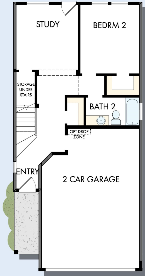
OPTIONAL BEDROOM 3 AT STUDY
