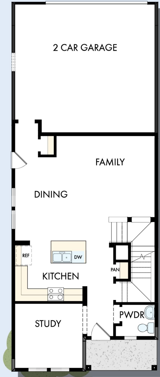
FIRST FLOOR
