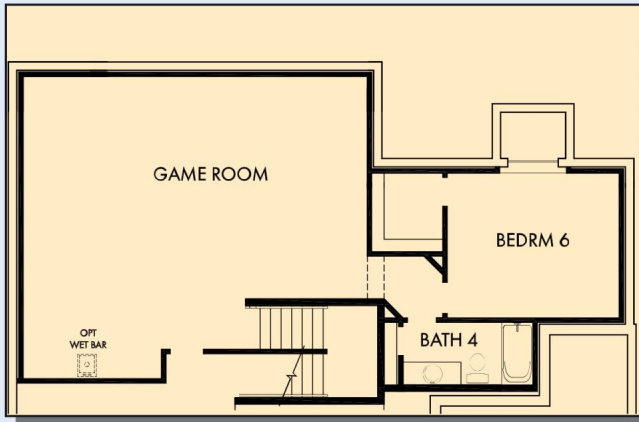
OPTIONAL GAME ROOM WITH BEDROOM 6 AND BATH 4 AT BASEMENT
