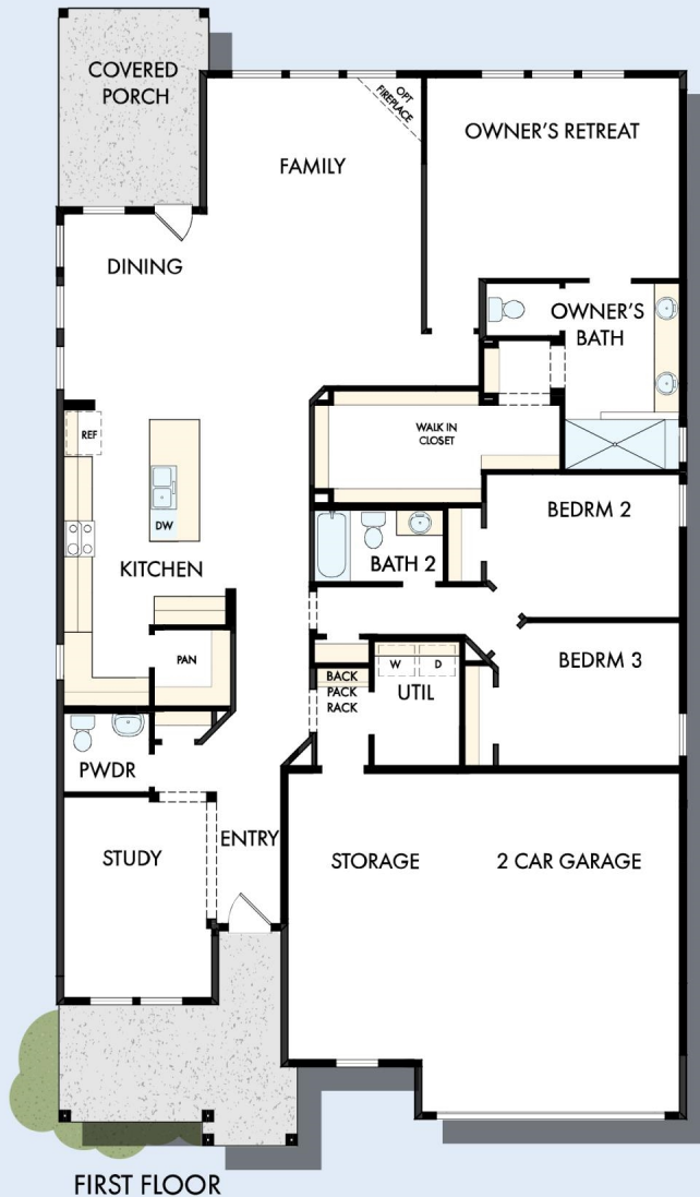
FIRST FLOOR WITH OPTIONAL SECOND FLOOR ATTIC STORAGE
