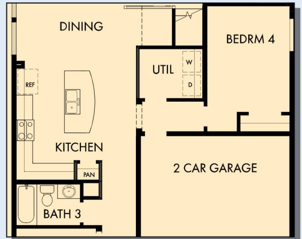
OPTIONAL BEDROOM 4 WITH BATH 3 AT GARAGE
