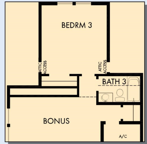
OPTIONAL BEDROOM 3 WITH BATH 3 AT THIRD FLOOR BONUS
