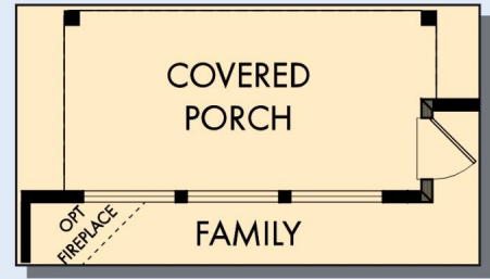
OPTIONAL COVERED PORCH AT FAMILY
