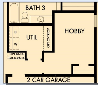
OPTIONAL HOBBY AT GARAGE
