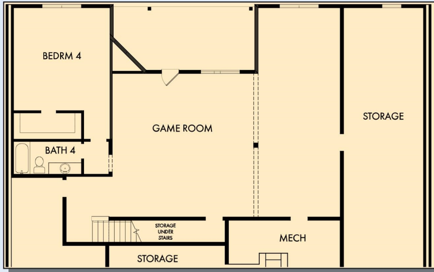
OPTIONAL BASEMENT WITH GAME ROOM, BEDROOM 4 AND BATH 4
