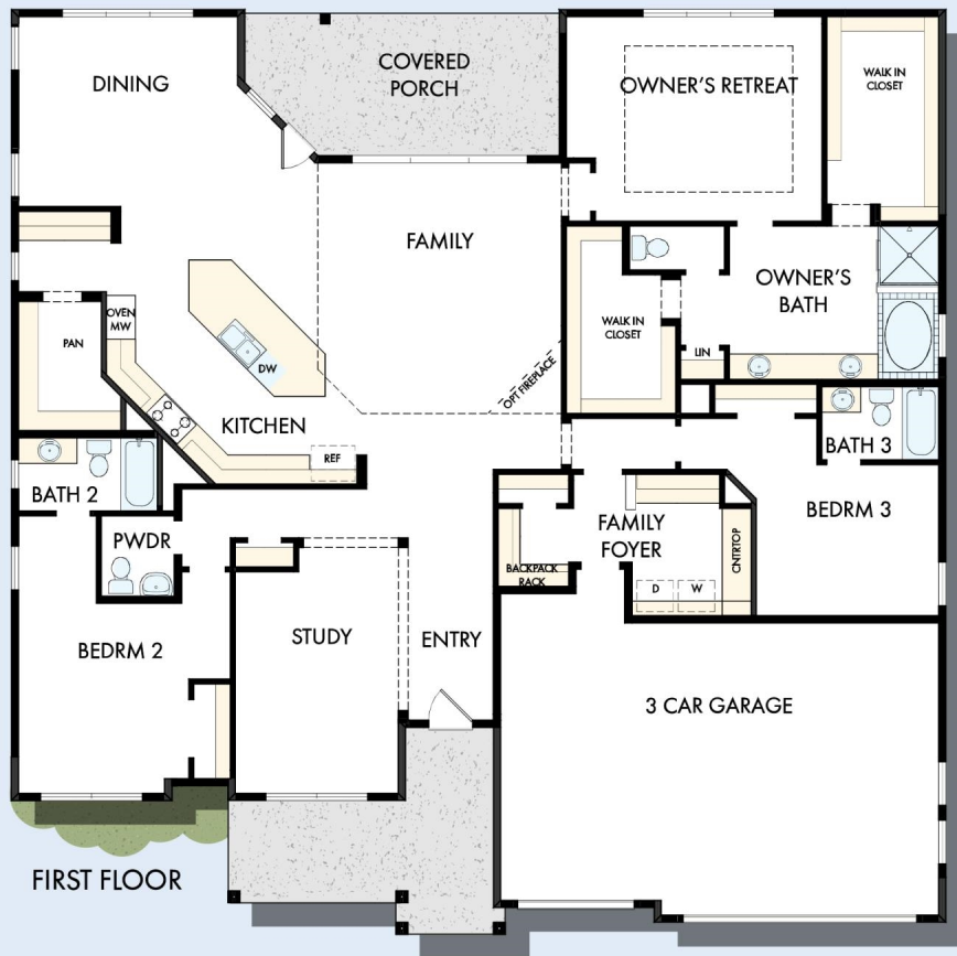
FIRST FLOOR WITH OPTIONAL BASEMENT
