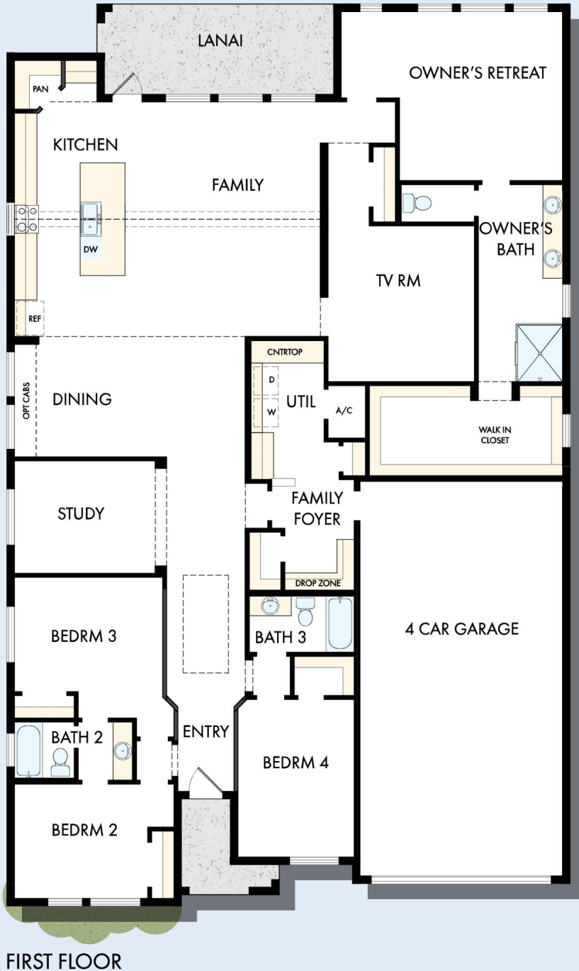
FIRST FLOOR WITH OPTIONAL SECOND FLOOR BONUS
