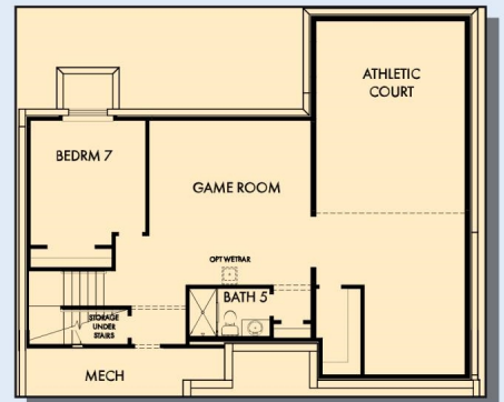
OPTIONAL GAME ROOM, BEDROOM 7 AND BATH 5 WITH ATHLETIC COURT AT BASEMENT
