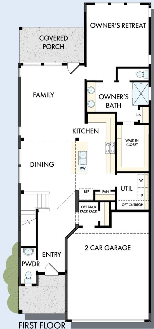
OPTIONAL EXTENDED COVERED PORCH AT FAMILY
