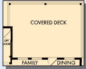
OPTIONAL EXTENDED COVERED DECK WITH BASEMENT
