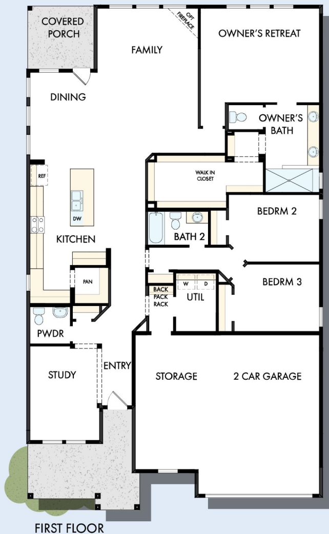
FIRST FLOOR WITH OPTIONAL SECOND FLOOR ATTIC STORAGE
