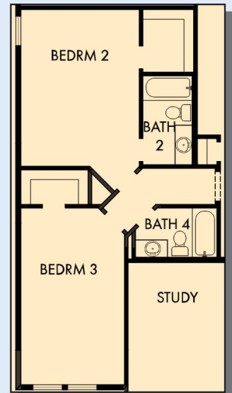
OPTIONAL EXTENDED BEDROOM 2 AND 3 WITH BATH 2 AND 4
