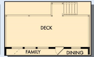
OPTIONAL EXTENDED DECK WITH WALKOUT BASEMENT
